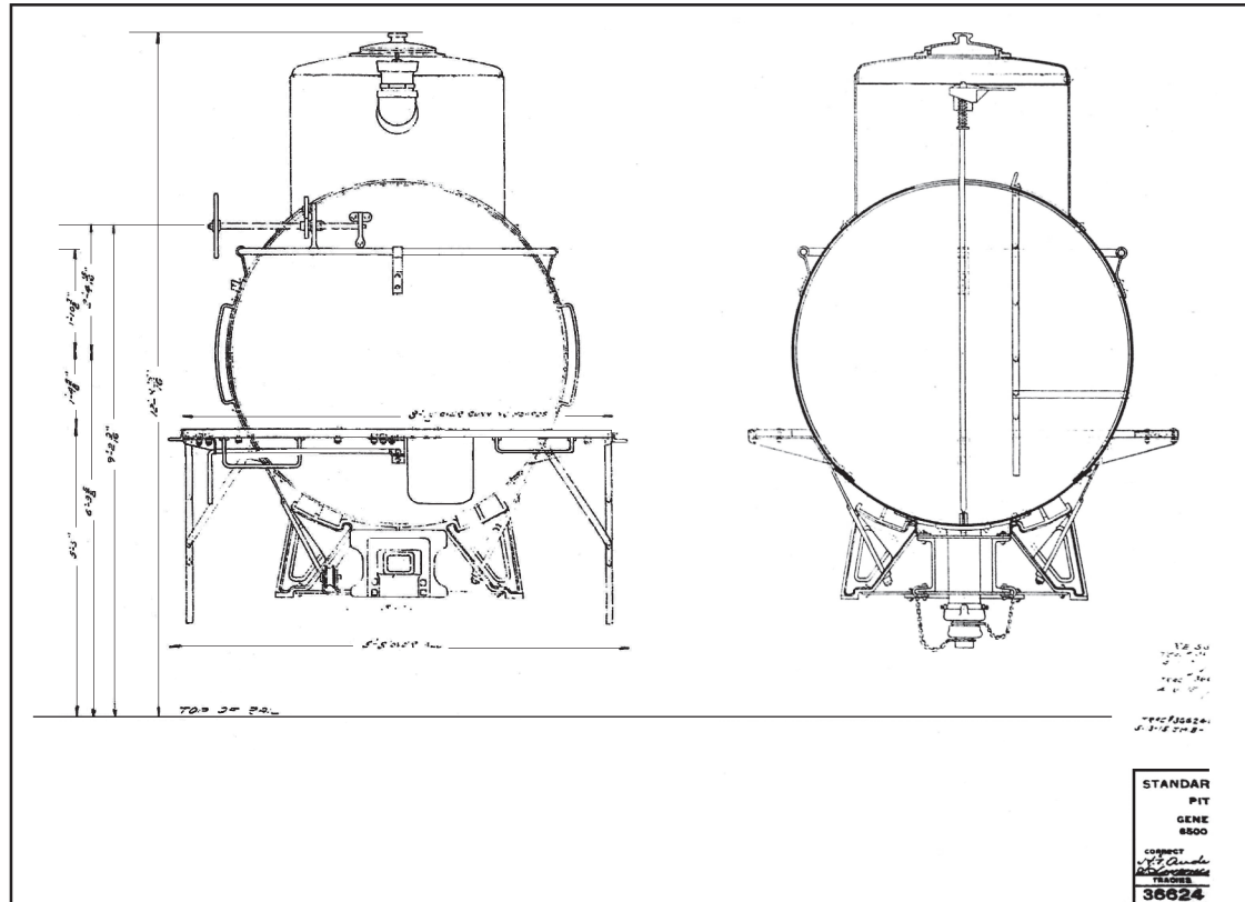
UTLX Class X 6,500 Gallon Tank Car GA Drawing April 22, 1915 Scale: 1/4 inch = 1 foot
